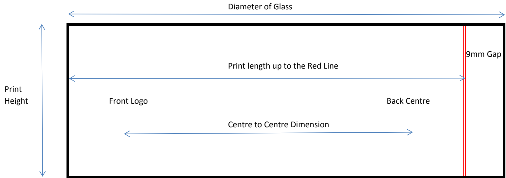
Colorlites Print Template. Where a tapered product is printed the mid diameter is taken as the diameter of Glass
